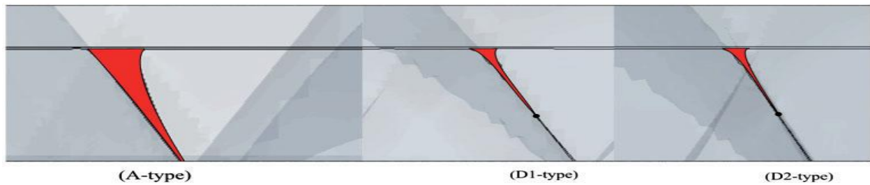
Figure 4. Blowhole of three kinds of rotors[9]
