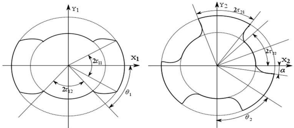
Figure 3. Generation of D-type rotor profile[2]
