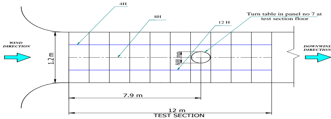
Fig. 2: Schematic showing concentration measurements for pre-selected lateral width in EWT for the double storied buildings model
