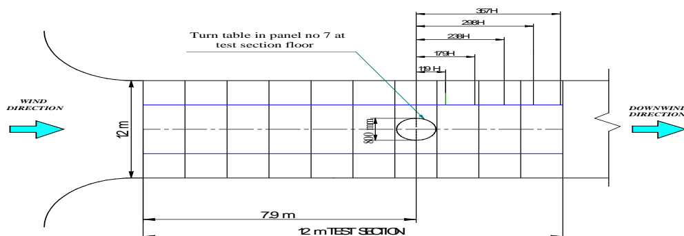
Fig. 1: Schematic showing downwind distances for tracer gas concentration measurement in the EWT
