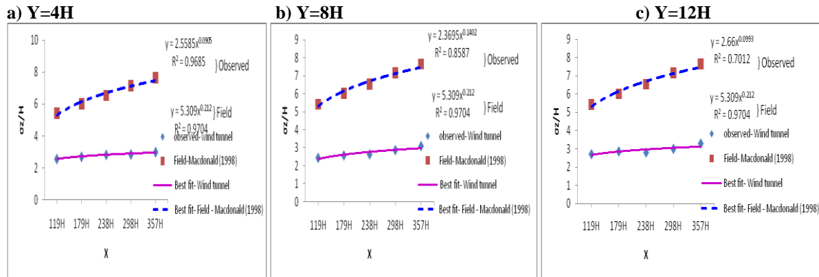
Fig. 9: Comparison of \sigma_z values for double storied inline array configuration with field data.
