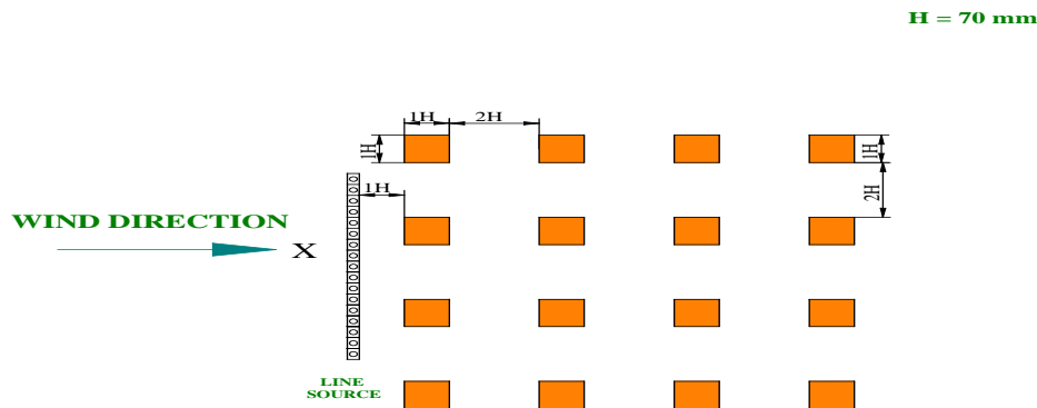
Fig. 4. Plan view of experimental buildings model inline array arrangement for double storied buildings
