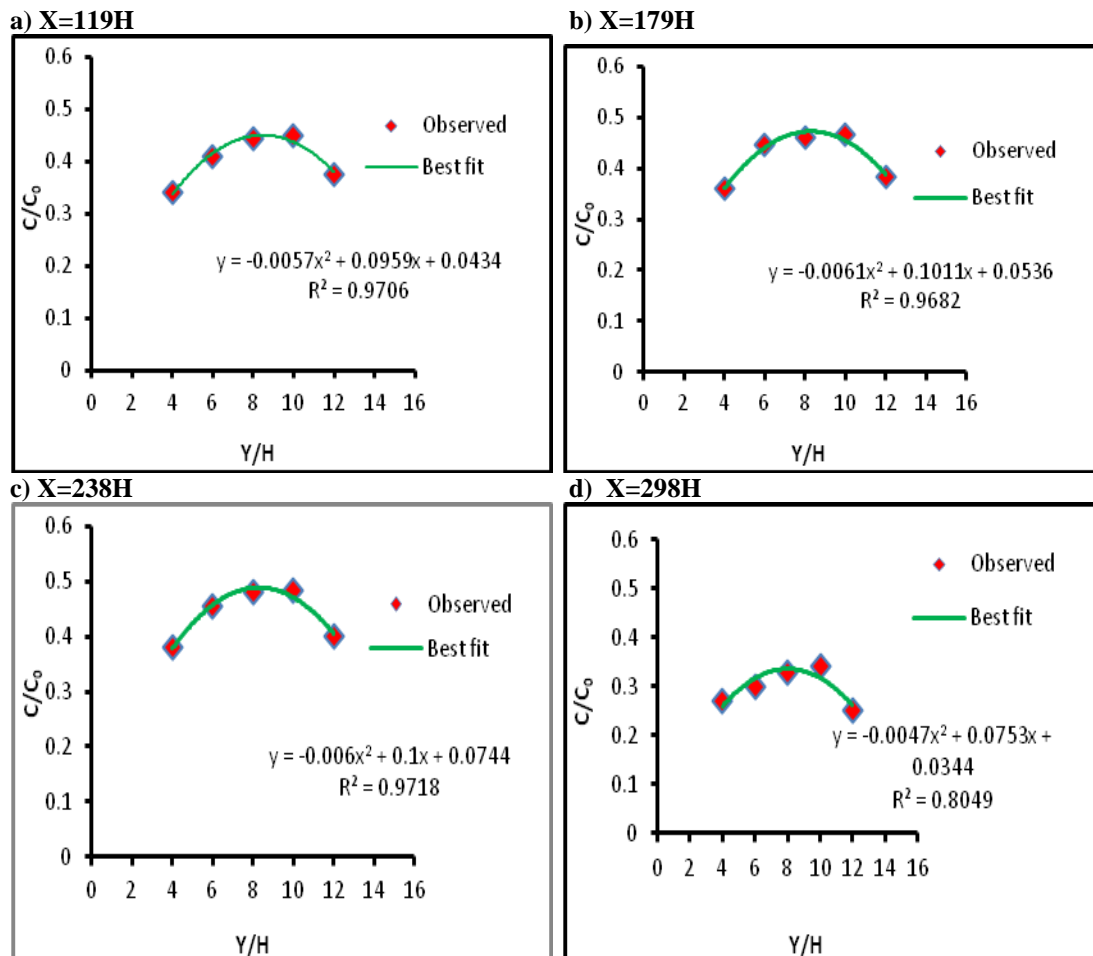
Fig. 5 Concentration profiles for 95°-orientation of line source for double storied buildings model configuration at Z/H=5.7.
