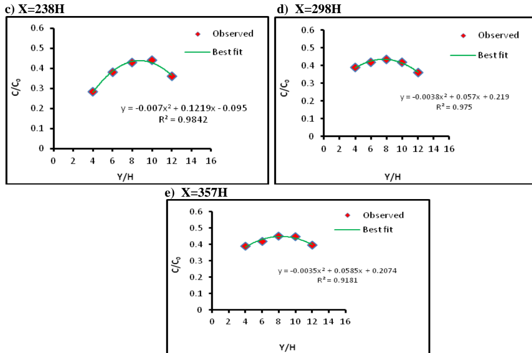
Fig. 5 Concentration profiles for 95°-orientation of line source for double storied buildings model configuration at Z/H=5.7.
