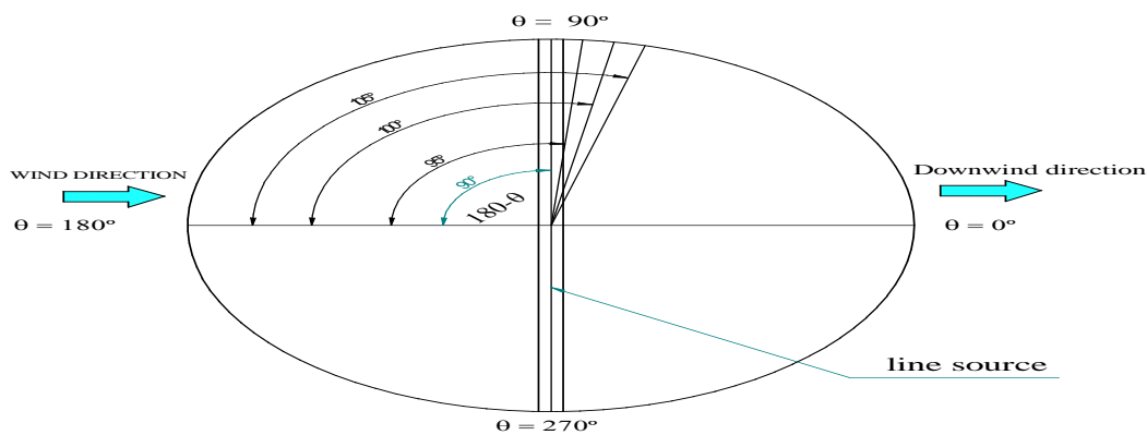
Fig. 3: Orientation of line source with respect to wind flow
