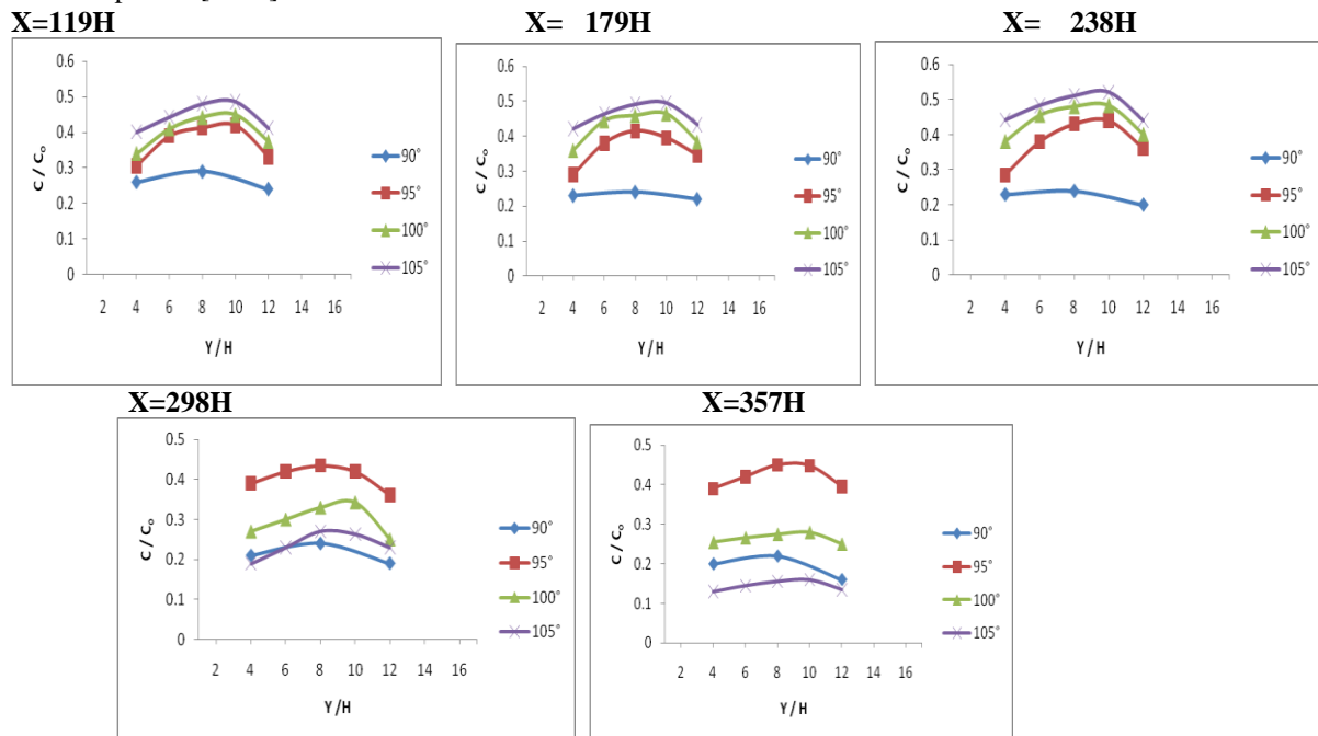
Fig. 8: Comparison of lateral concentration profiles for selected wind direction
