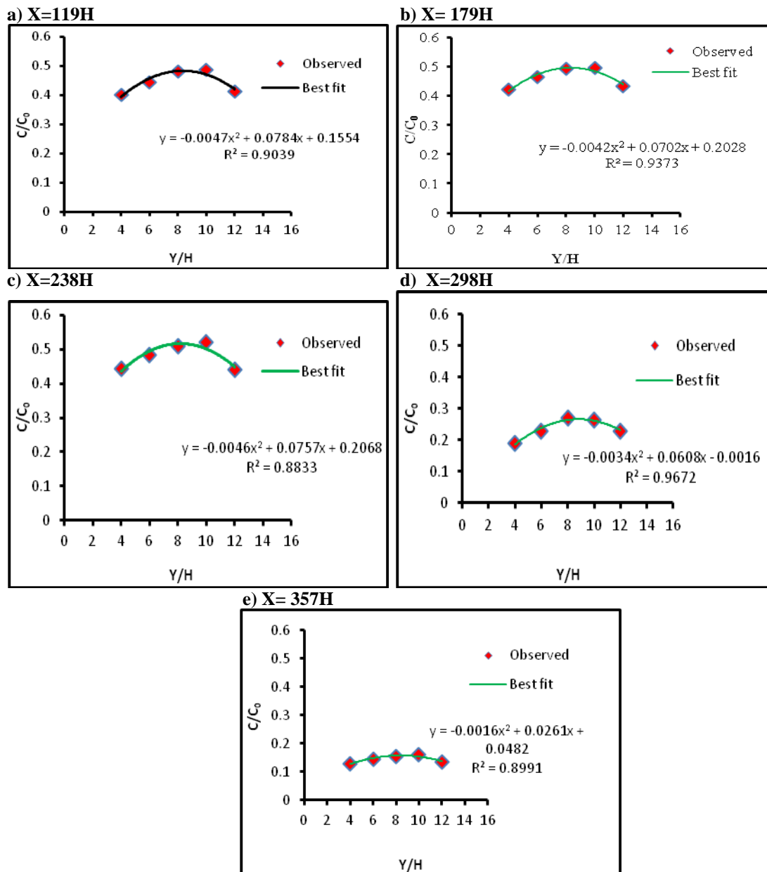
Fig. 7. Concentration profiles for 105°-orientation of line source for double storied buildings model configuration at Z/H=5.7
