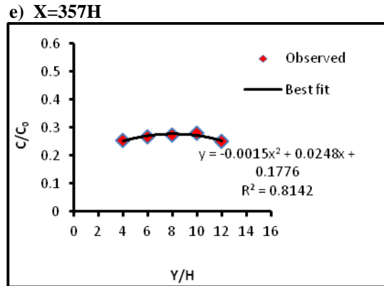
Fig. 6. Concentration profiles for 100°-orientation of line source for double storied buildings model configuration at Z/H=5.7
