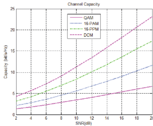
Fig 11: Channel Capacity vs SNR
