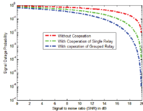
Fig 12: Outage Probability vs SNR
