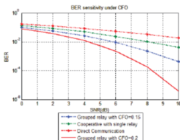
Fig 14: BER Sensitivity under CFO
