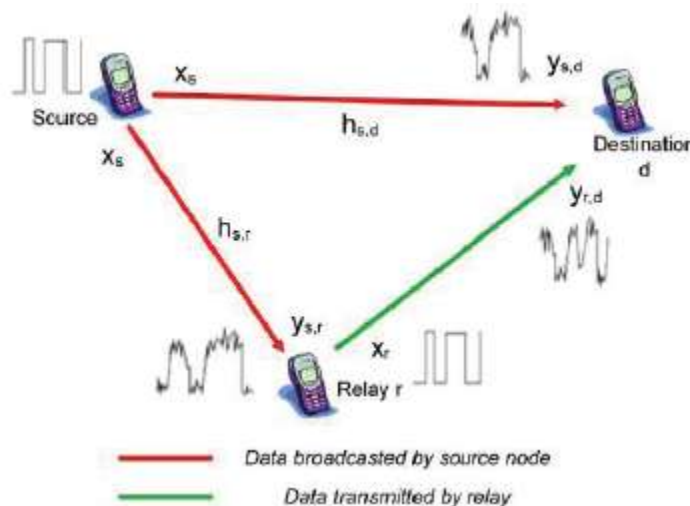
Fig 4: Decode and Forward Model
