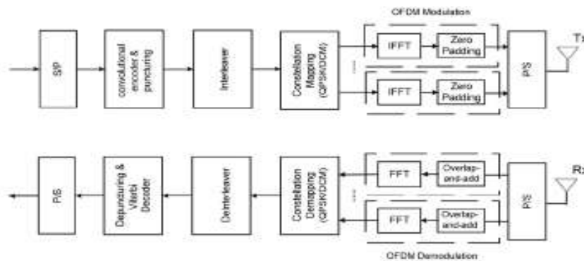
Fig 6: Structure of MB ofdm UWB
