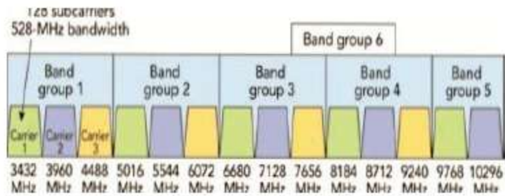
Fig 5: Band Group Allocation
