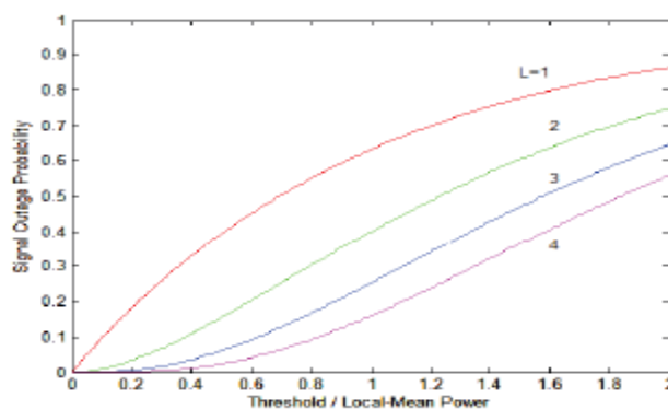
Fig 13: Outage Probability vs Threshold/local-mean power
