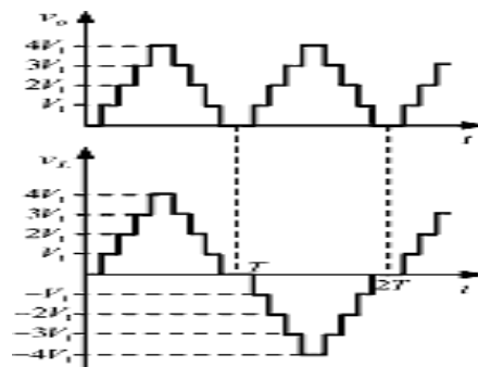
Fig 3 Output waveform of H-bridge
