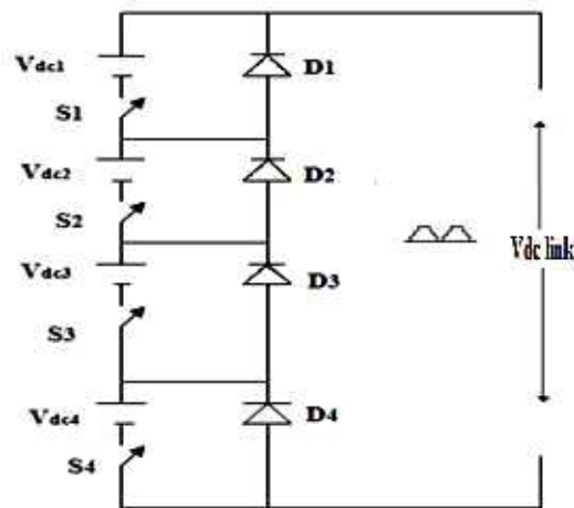
Fig 2(a) Proposed bypassed diode technique
