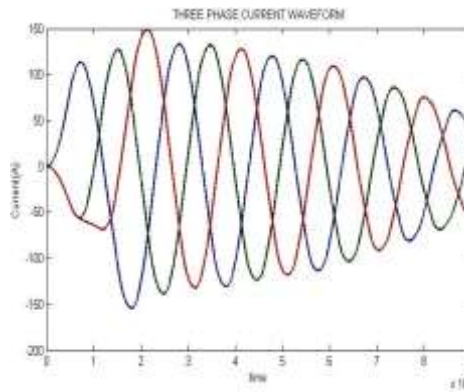
Fig 6 Three phase current waveform
