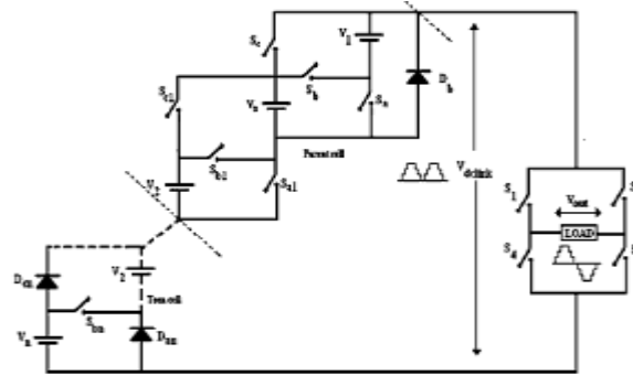
Fig 1(a) Basic unit suggested in[6]
