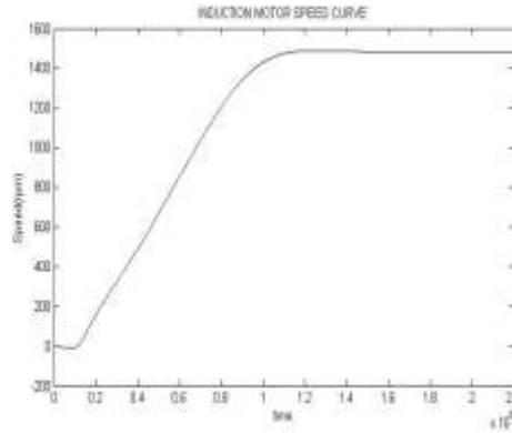
Fig 7 Proposed inverter fed Induction motor speed curve
