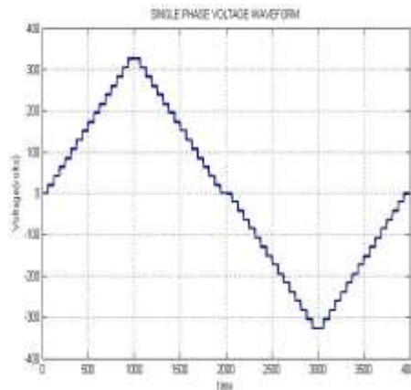
Fig 4 single-phase output voltage
