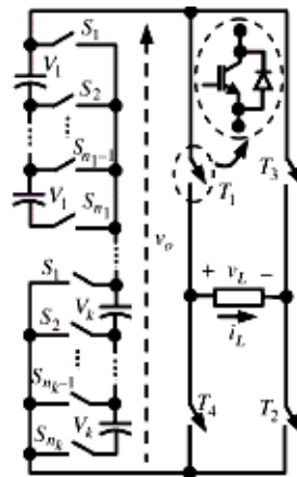
Fig 1(b) Basic unit suggested in[7]
