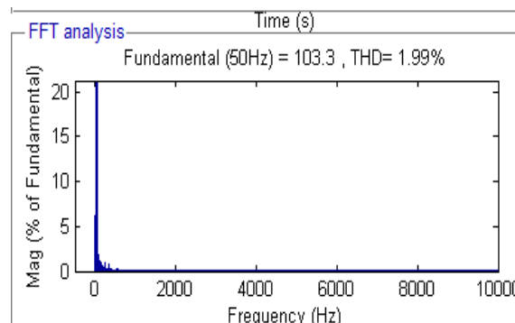
Fig 8 THD waveform
