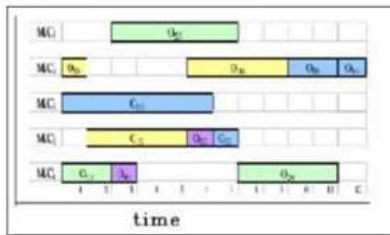
Figure 2: Gantt chart of operation on machines Modelling of flexible manufacturing system
