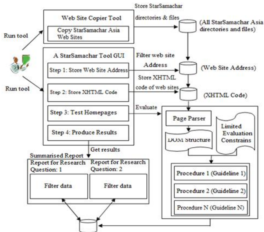
Figure 1 WebUSA tool architecture
