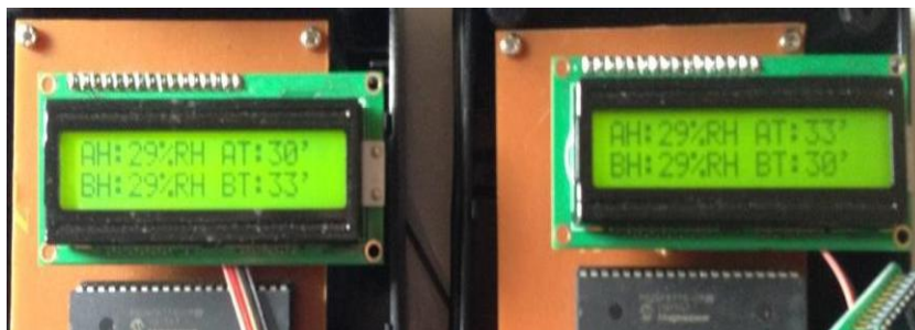
Figure 7. Humidity &amp; Temperature Reading at the transmitter and receiver.
