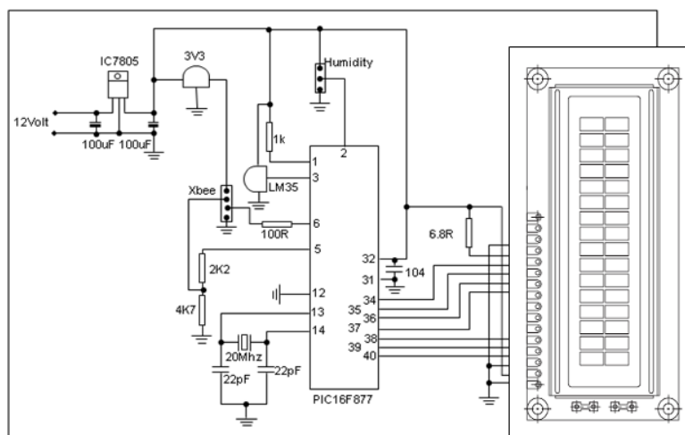
Figure 5. LCD Interface with PIC Microcontroller
