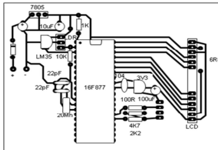
Figure 4. Transmitter & Receiver Circuit Printing Layout
