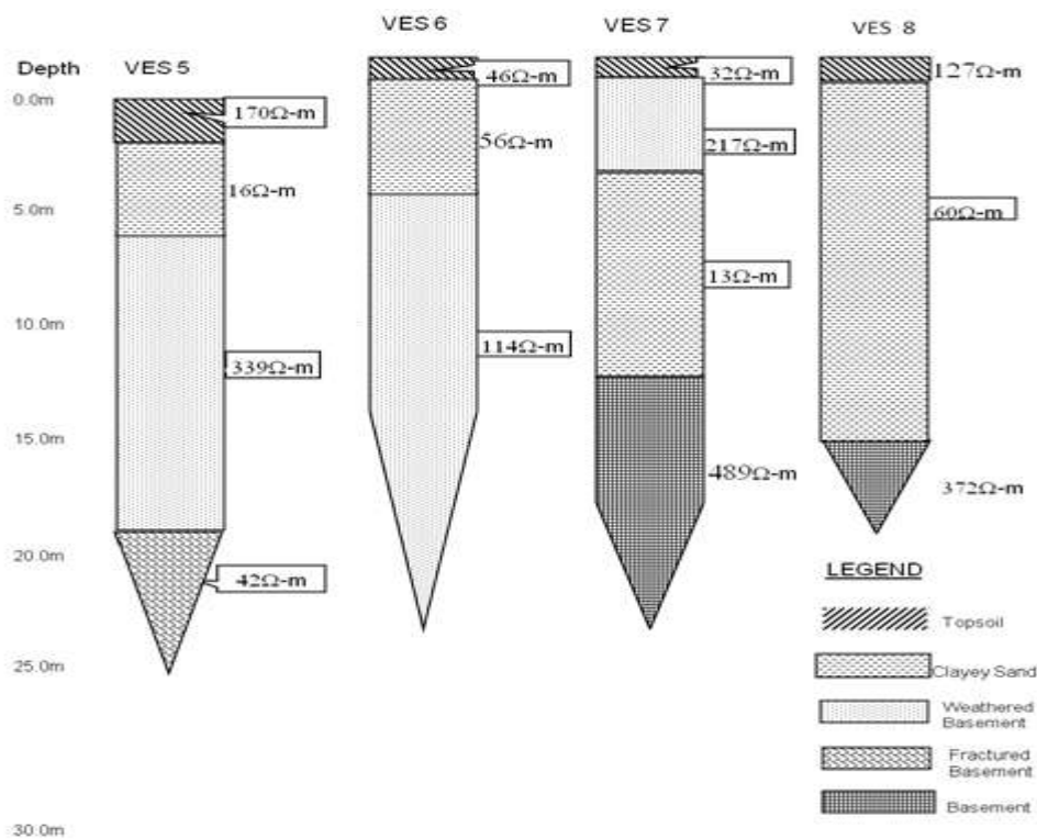
Fig. 3b: Geoelectric Section of VES 5 - 8.
