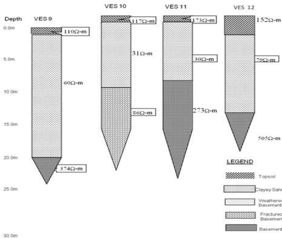
Fig. 3c: Geoelectric Section of VES 8 - 12.
