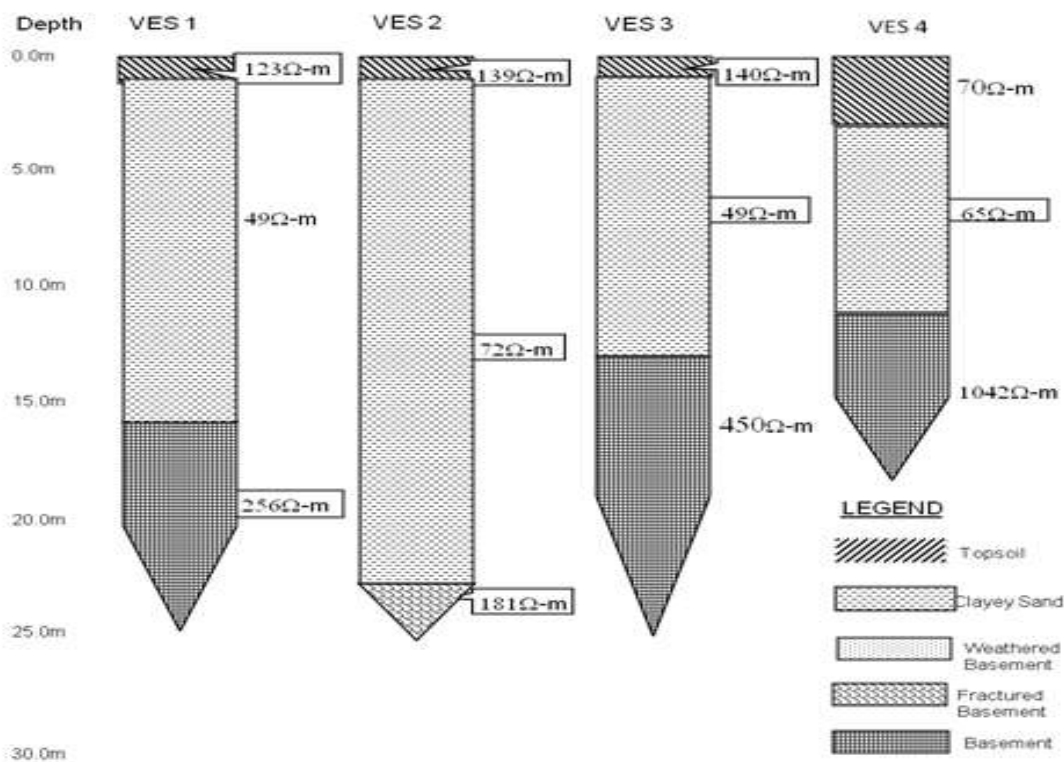
Fig. 3a: Geoelectric Section of VES 1–4.
