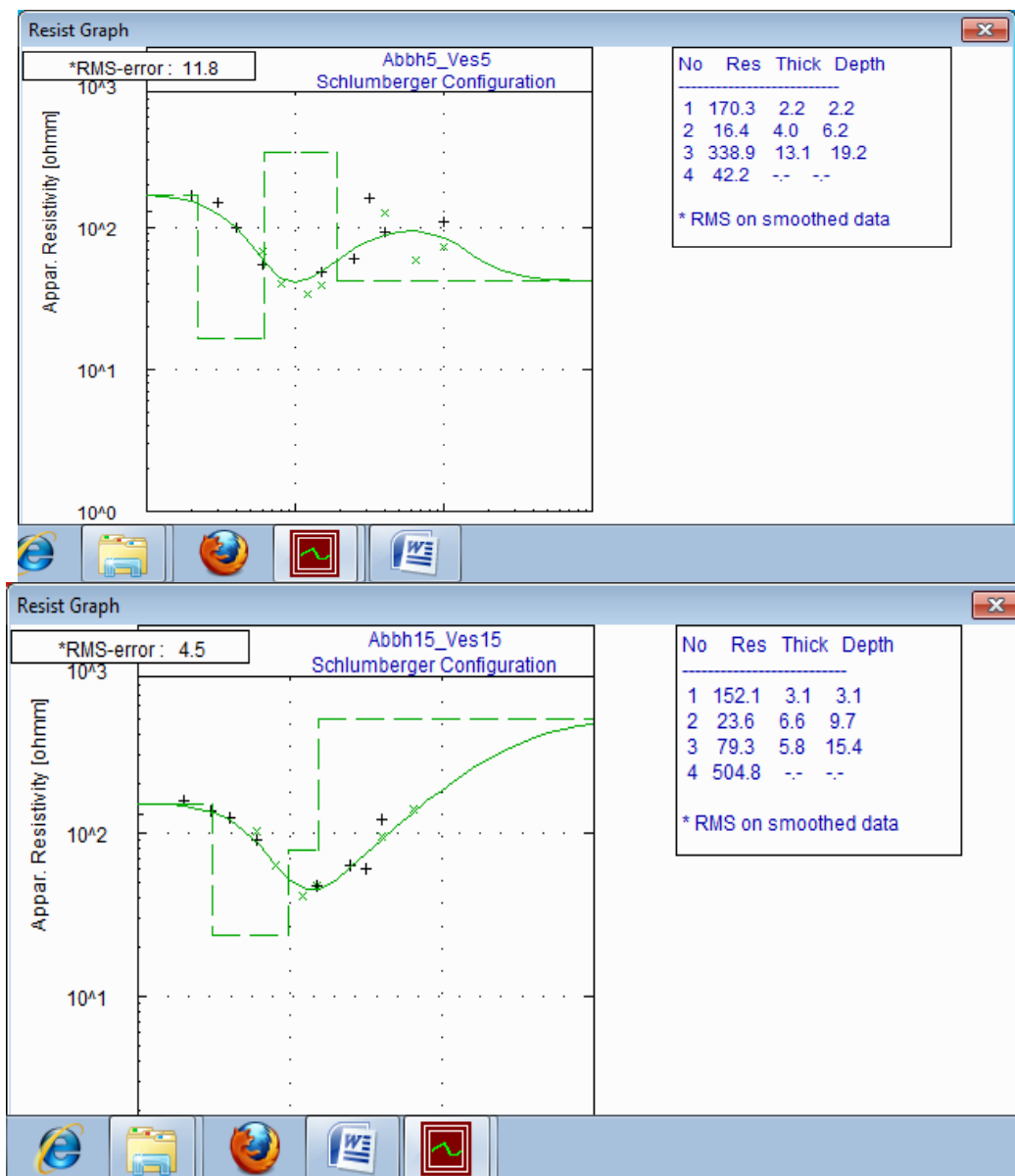
Fig. 2. Typical Geoelectric curves from the study area
